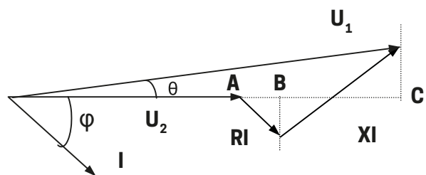
Diagrama vectorial
